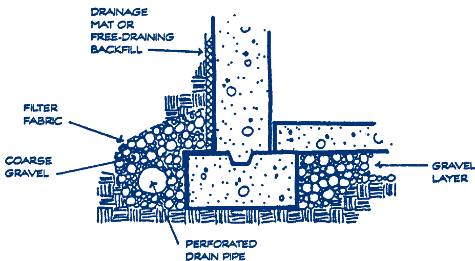
Figure 6: Hydrostatic pressure relief.
