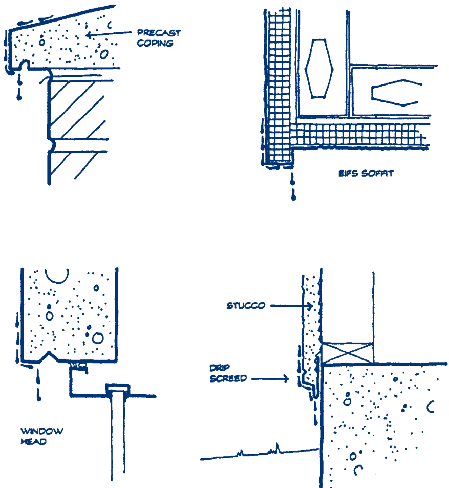
Figure 4: Drips break surface tension.
