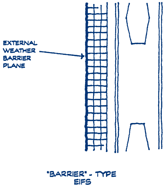
Figure 7: Rain barrier type systems.
