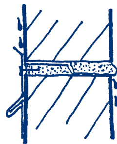
GRAVITY
