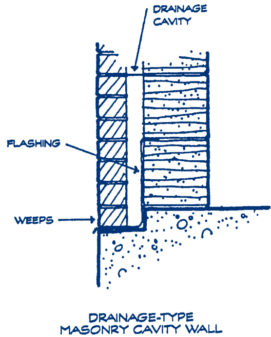
Figure 8: Drainage type systems.
