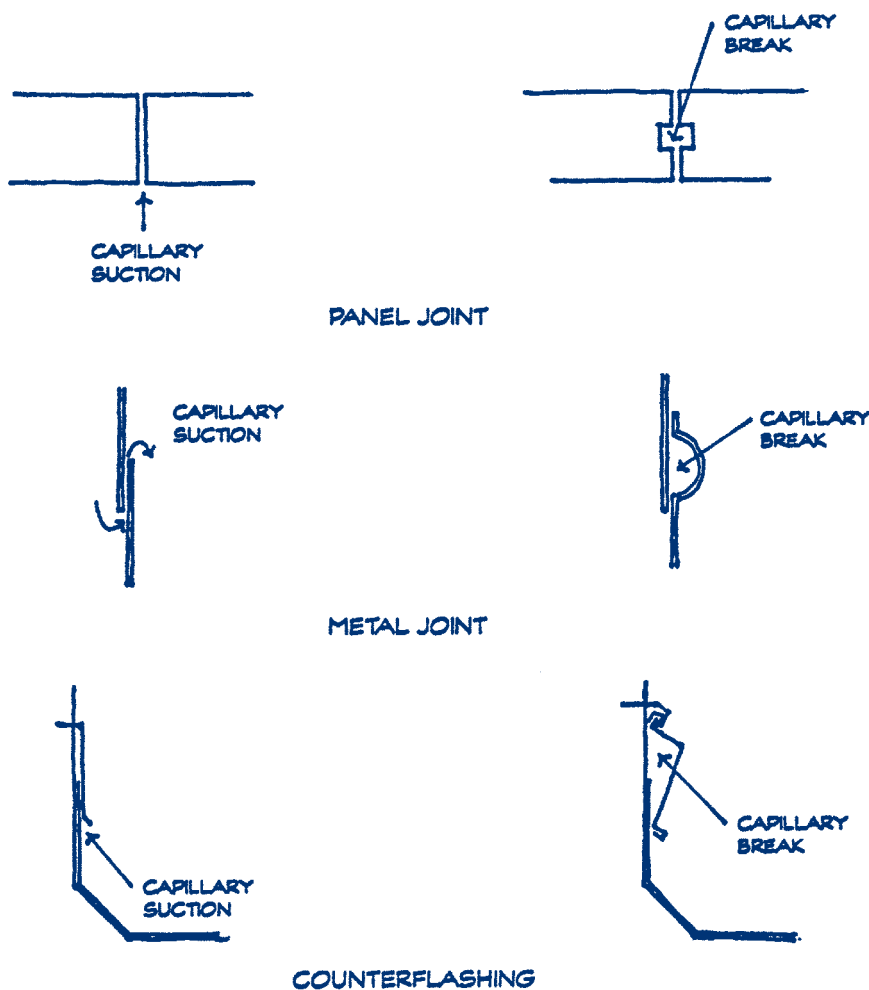
Figure 5: Capillary breaks prevent suction.
