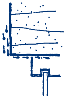
SURFACE TENSION
