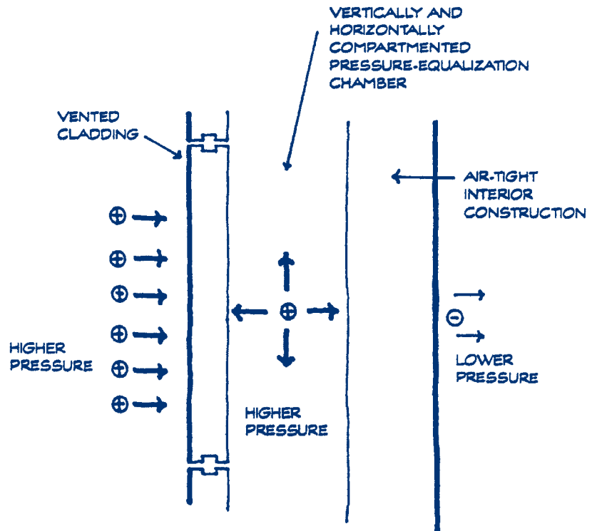
Figure 9: Rain screen system concept.
