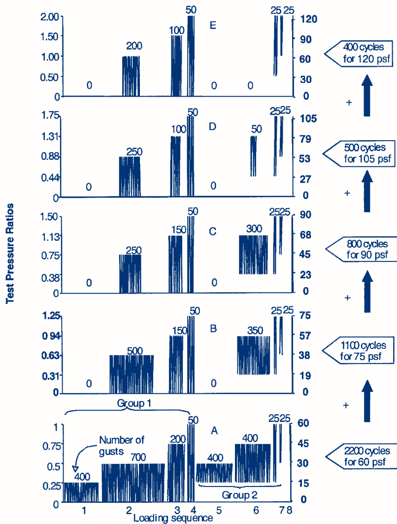
Figure 3. SIGDERS dynamic wind test protocol.
