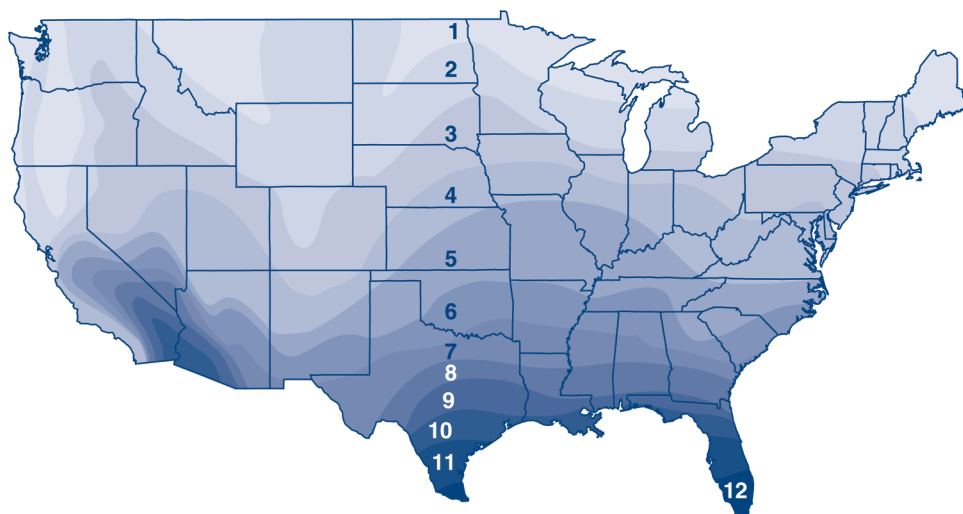
Figure 1: U.S. climate Region Map, Cooling Reprinted from Energy Star Consumer Investment Information, U.S. EPA, October, 1998.
