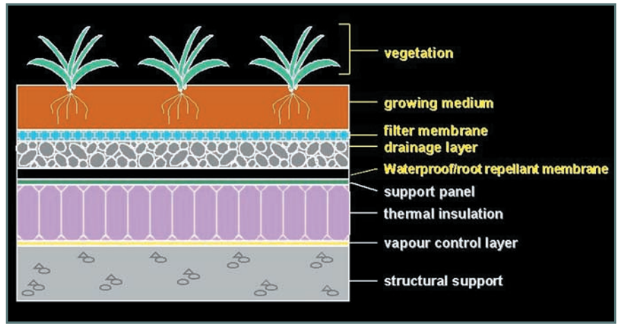
Figure 2: General elements of a green roof system. Source: National Research Council, Institute for Research in Construction No. 1. Developed by Steven Peck, Stephanie Tenzer, and Dr. Brad Bass.
