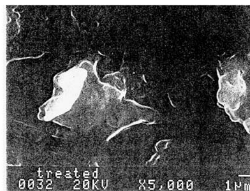
Figures 3 and 4: Microphotographs of treated and untreated new EPDM membranes.
