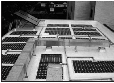
Figure 5 - Open-energy photovoltaic module and single-ply membrane system.
