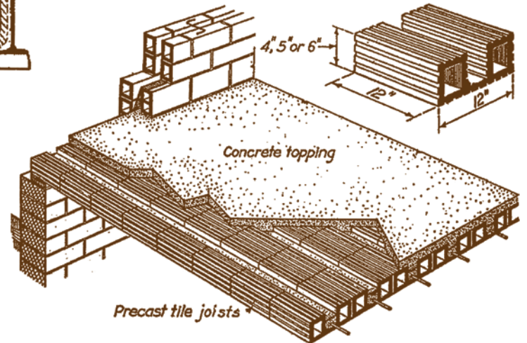
Figure 2 – Typical combination clay tile and integral concrete topping roof-deck system.
