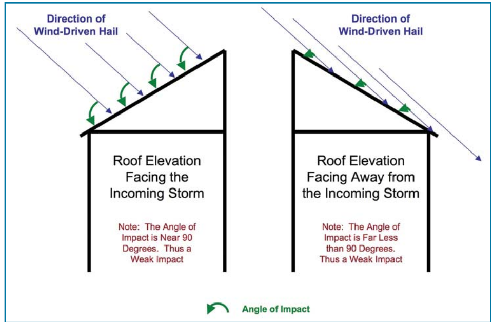
Figure 4 – Hail impact on roof facing incoming storm and roof facing away from incoming storm.
