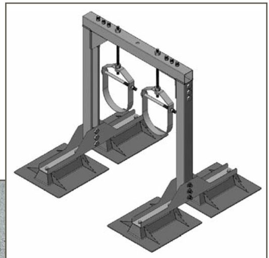
Figure 12 – Typical pre-manufactured pipe support detail.
