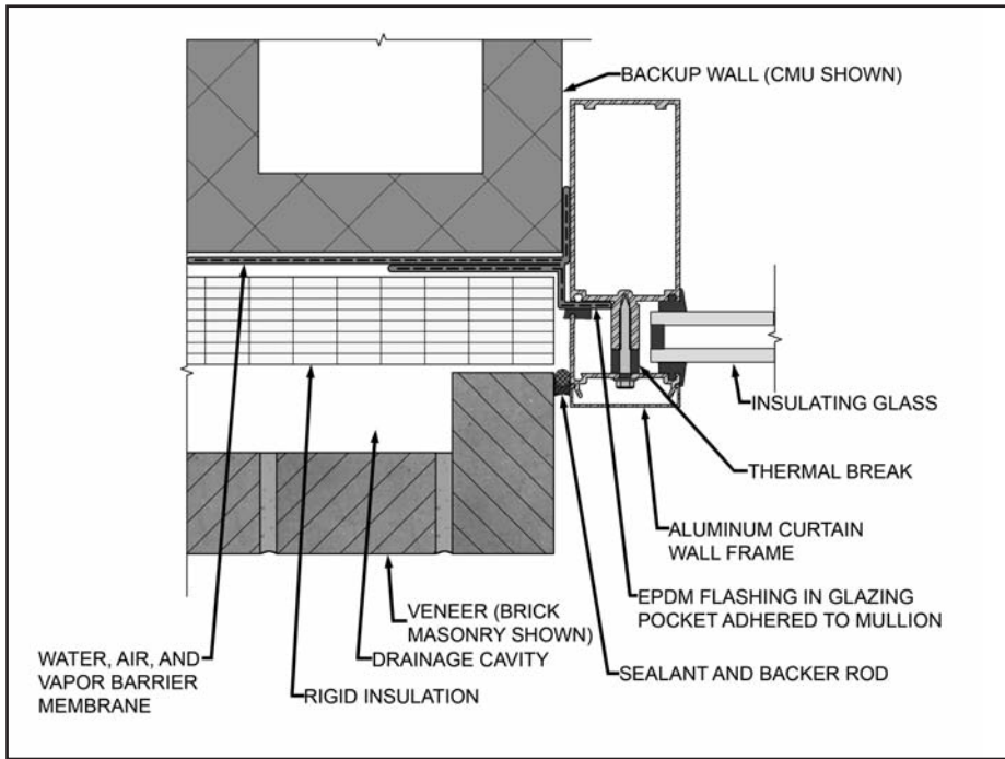
Figure 6 – Integration of water, air, and vapor barriers with curtain wall frame and alignment of thermal barrier.
