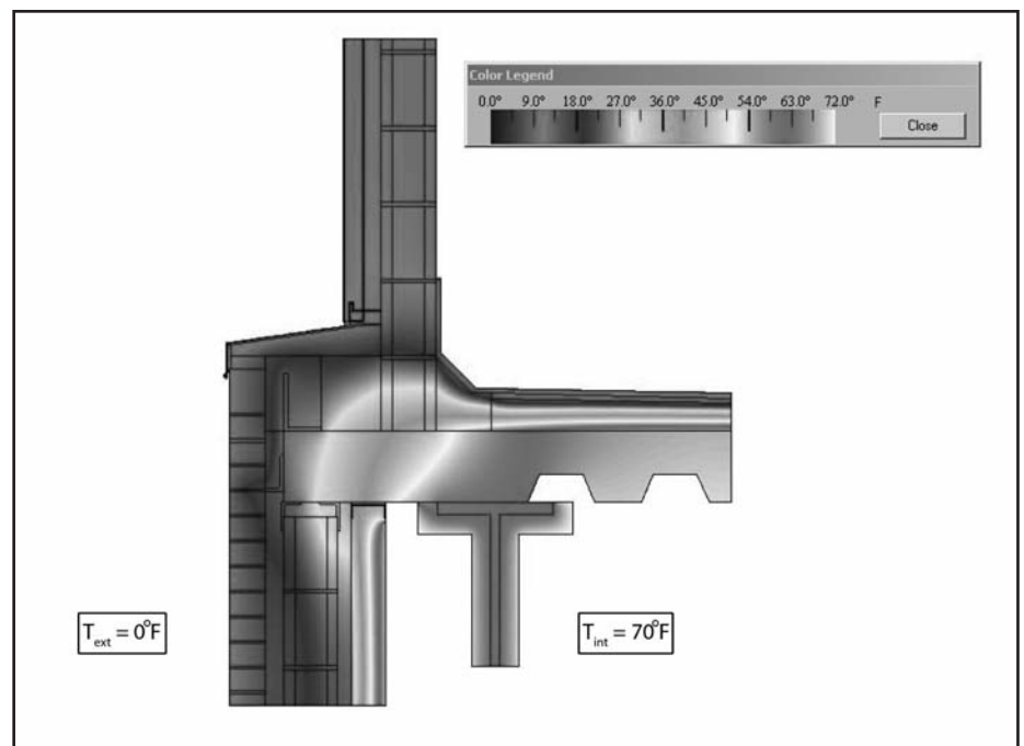
Figure 7 – Thermal gradients at a masonry parapet.
