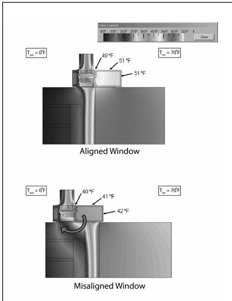
Figure 3 – Thermal gradients of aligned and misaligned windows.
