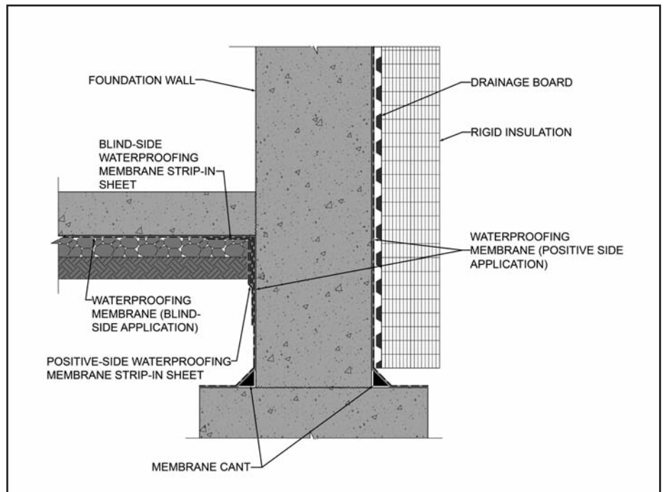
Figure 8 – Below-grade membrane waterproofing.
