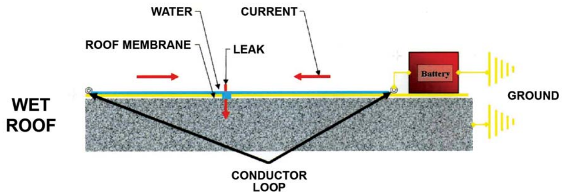
Figure 1 – The surface of the waterproofing must be wetted to provide an electrically conductive medium.
