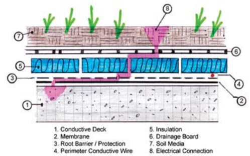
Figure 4 - ELD section with overburden in place.
