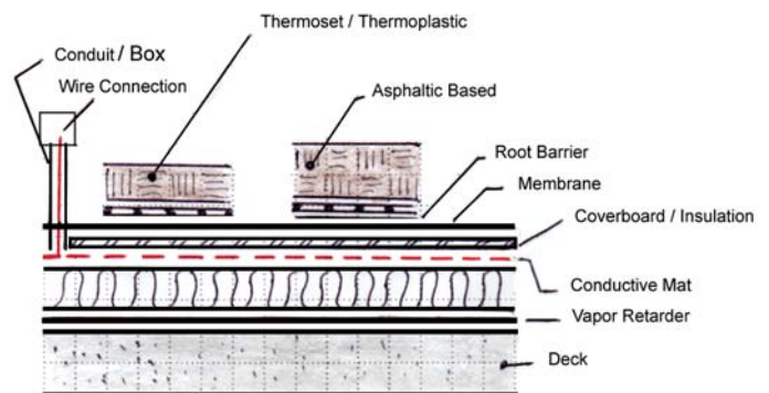
Figure 3 - Testing at nonconductive decks or conductive decks with vapor retarders.
