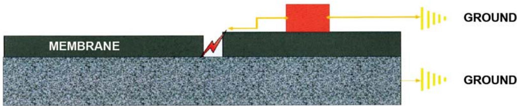
Figure 2 – The power source is grounded to the conductive deck, with the membrane acting as insulator.
