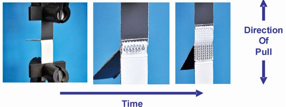
Figure 4 – T-peel test showing delamination between cap and core membrane plies, thereby indicating lamination strength.
