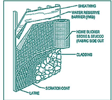
Photo 27 — Drainage membrane over WRB (courtesy Benjamin Obdyke).
