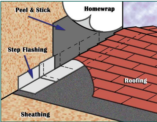
Photo 15 – Peel-and-stick flashing from sheathing onto metal flashing.
