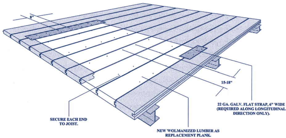
Figure 6 – Repairs are probably best made by replacement in kind, although tongue-and-groove integrity must be maintained. Any variations of the repair depicted must recognize this aspect.
