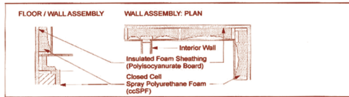
ASSEMBLY C: ccSPF DOUBLE-INSULATED APPLICATION
