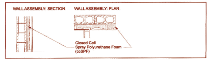
ASSEMBLY D: INTERIOR ccSPF APPLICATION
