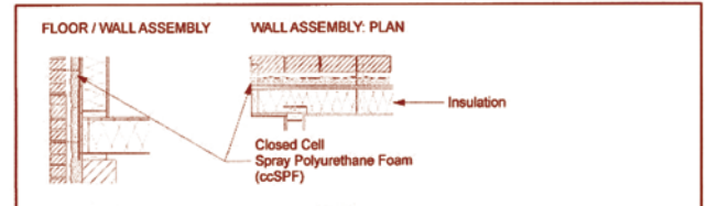
ASSEMBLY B: EXTERIOR ccSPF APPLICATION
