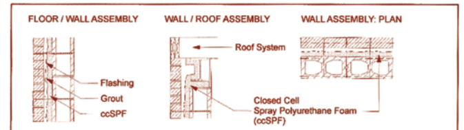
ASSEMBLY E: EXTERIOR ccSPF APPLICATION
