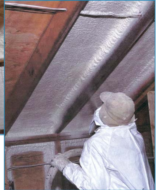
Photos 5 and 6 – Closed-cell foam should be installed in a “picture frame” technique to ensure uniform installation and to enhance adhesion to the studs.
