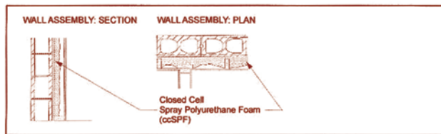
ASSEMBLY D: INTERIOR ccSPF APPLICATION
