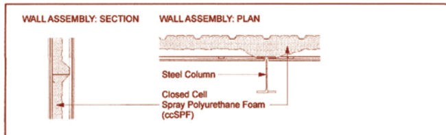
ASSEMBLY F: INTERIOR ccSPF APPLICATION
