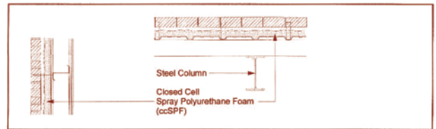
ASSEMBLY G: EXTERIOR ccSPF APPLICATION
