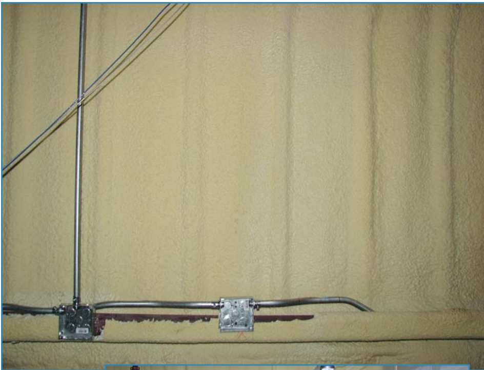
Photos 3 and 4 – Here, ccSPF is installed on the interior of a metal building without wall studs. This type of application has an added benefit of reducing thermal bridging through the metal beams and columns.
