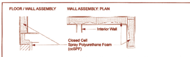
ASSEMBLY A: INTERIOR ccSPF APPLICATION
