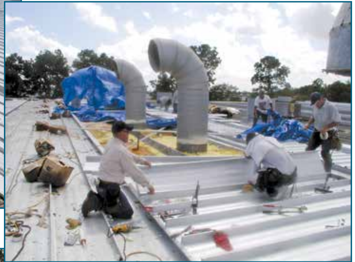
Figure 14 – Installing transverse panels around large round pipe penetrations.
