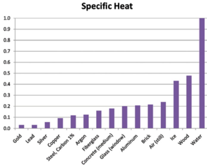
Figure 6 – Heat capacity of various materials in Btu/lb. °F.
