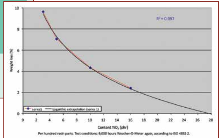
Figure 4 – Weight loss vs. \text{TiO}_2 levels.
