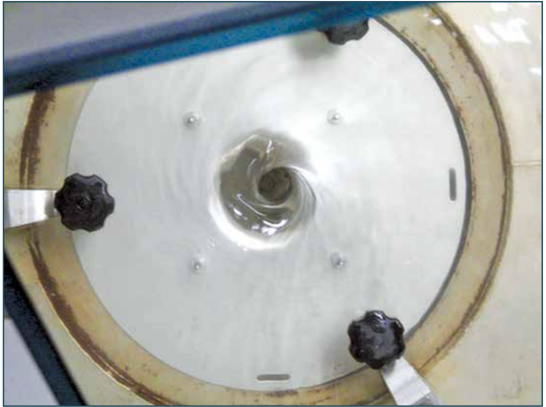
Figure 4 – This image of a roof drain within a drain flow test rig clearly shows the vortex fully formed, which can significantly slow the speed of water flowing through a drain fixture.
