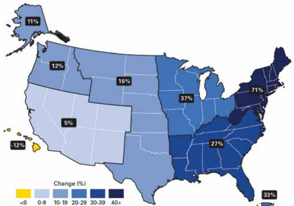
Figure 1 – Map shows percentage increases in the amount of precipitation falling in very heavy events (defined as the heaviest 1% of all daily events) from 1958 to 2012 for each region of the continental U.S., resulting in an increased number of microburst rainstorms with a significant amount of rain in a short period of time. Source: U.S. National Climate Assessment's "Climate Change Impacts in the United States," published in 2014.
