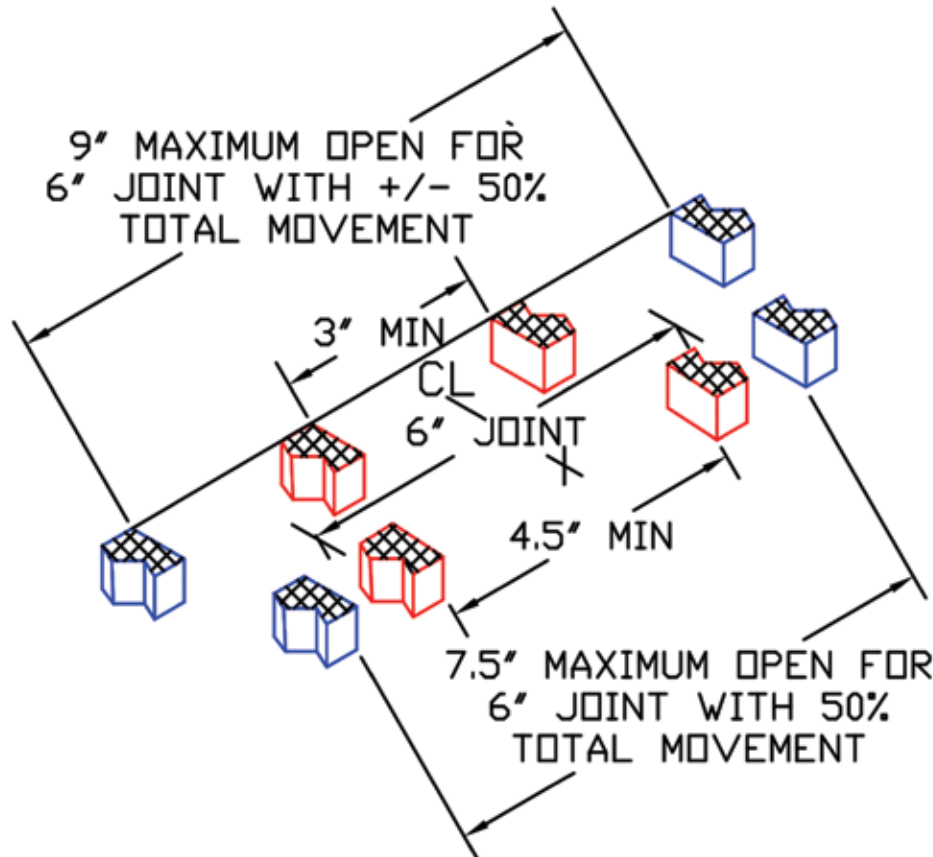
Figure 10 – Detail of a joint with two different movement references.
