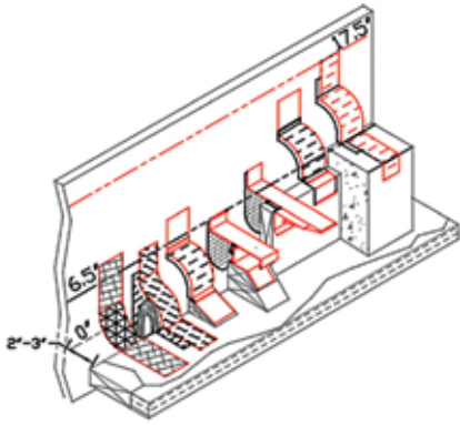
Figure 5 – Roof-to-wall joint closure styles.
