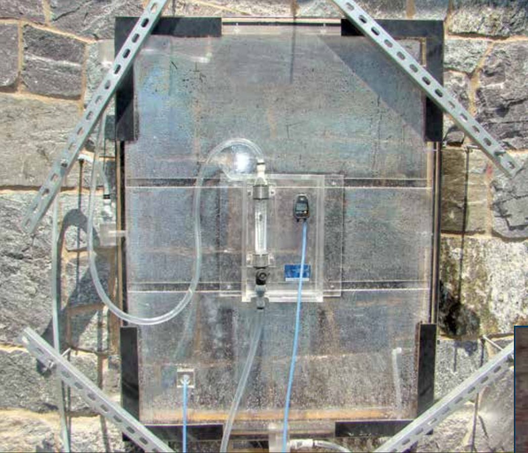
Photo 8 – Chamber securely anchored to masonry wall during an ASTM C1601 test.
