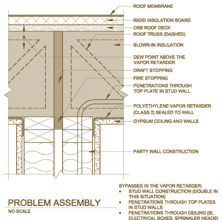
Figure 1 – Problem assembly.
