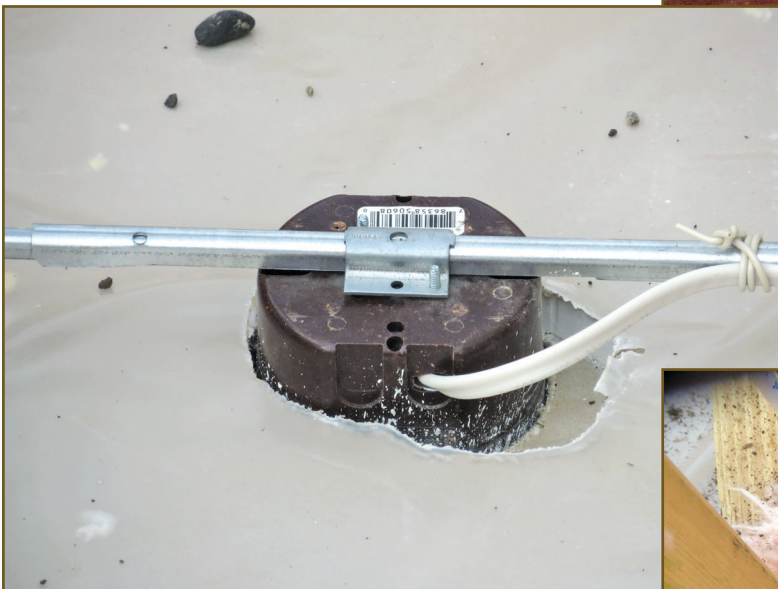
Figure 4 – Vapor retarder bypass at ceiling light electrical box.
