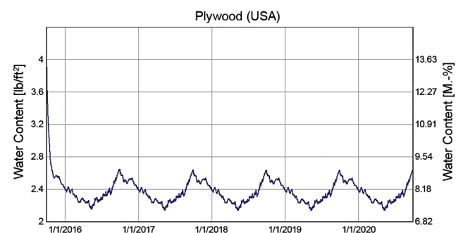
Figure 9 – Hygrothermal model graph of the plywood roof deck in the roof assembly shown in Figure 8.
