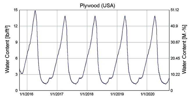
Figure 7 – Hygrothermal model graph of the roof deck in the roof assembly shown in Figure 1.
