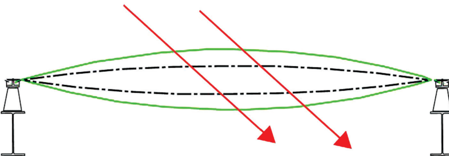
Figure 5 – Diagram sketch of a four-foil ETFE cushion (fritted foils shown as dashed lines) with higher pressurization between the second and third foil opening the frit pattern, allowing solar access during the winter months.
