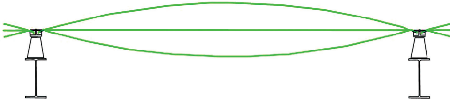
Figure 2 – A sketch diagram of a three-foil ETFE cushion.
