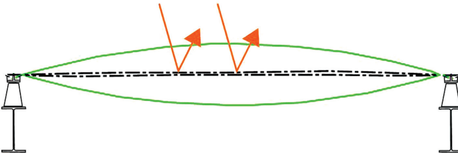
Figure 4 – Diagram sketch of a four-foil ETFE cushion (fritted foils shown as dashed lines) with lower pressurization between the second and third foil, closing the frit pattern and limiting solar access during the summer months.
