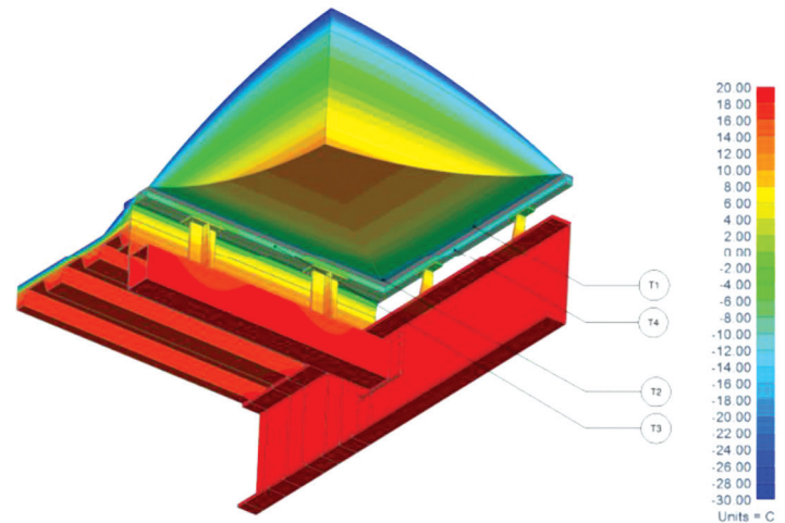
Figure 7 – 3-D thermal model of three-foil ETFE cushion in a northern climate at -22°F (-30°C).
