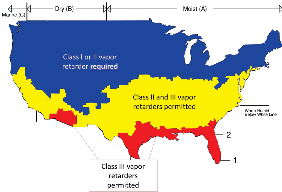
Figure 1 – General vapor retarder requirements per 2015 IBC Section 1405.3.1.
