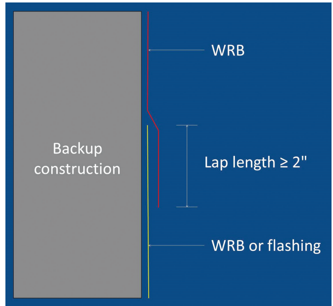
Figure 2 – Proper shingle lapping of WRBs.
