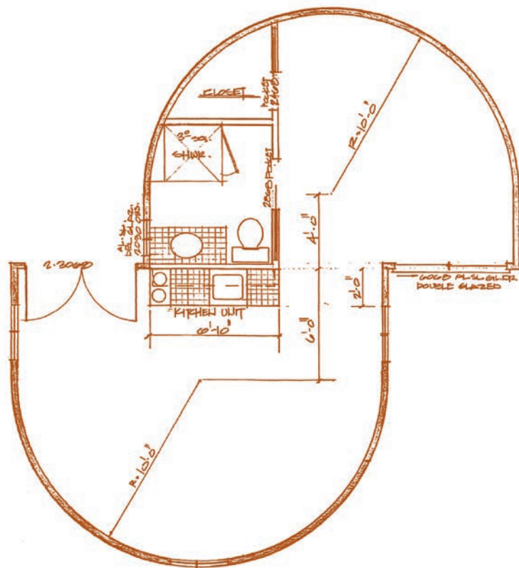
Floor plan by Ted Thoeny, PE.
