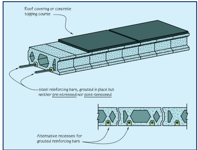
Figure 8 – Instead of seven-strand cable, ordinary rebar was used, so this manufacturing procedure was not as effective as modern pre-stressing or post-tensioning techniques; consequently, design tables for modern pre-stressed concrete product should not be used to analyze this type of roof deck.
