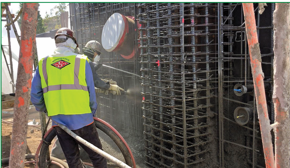
Figure 6 – Observations of the placement of shotcrete.
