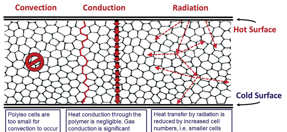
Figure 3 – Schematic showing the three main forms of thermal transfer through a closed-cell foam material.
