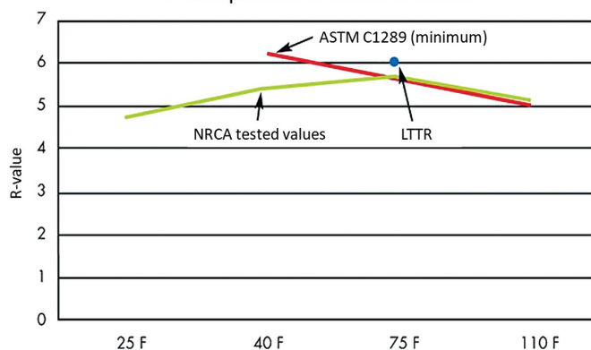
Figure 5 – Mean thermal resistance versus temperature for NRCA test of 16 polyiso samples, average values.
