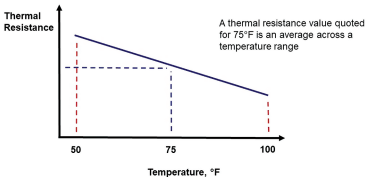
Figure 4 – Thermal resistance is not measured at a single temperature but across a gradient. In this case, the quoted 75°F value is an average between 50°F and 100°F.
