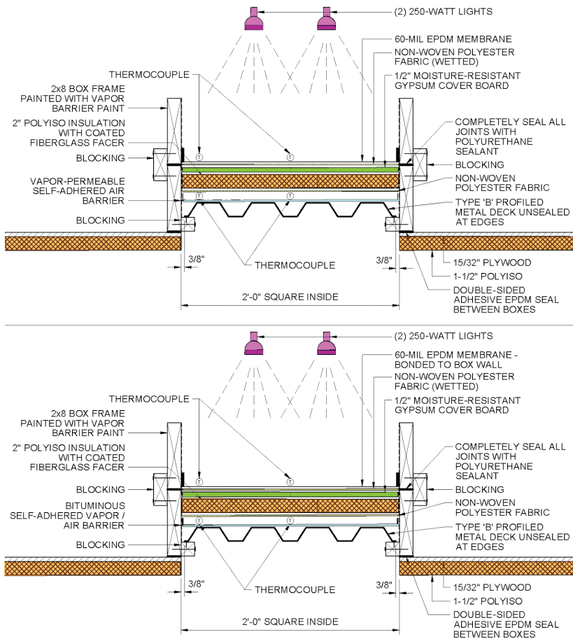
Figure 6 – Initial test panel assembly.
