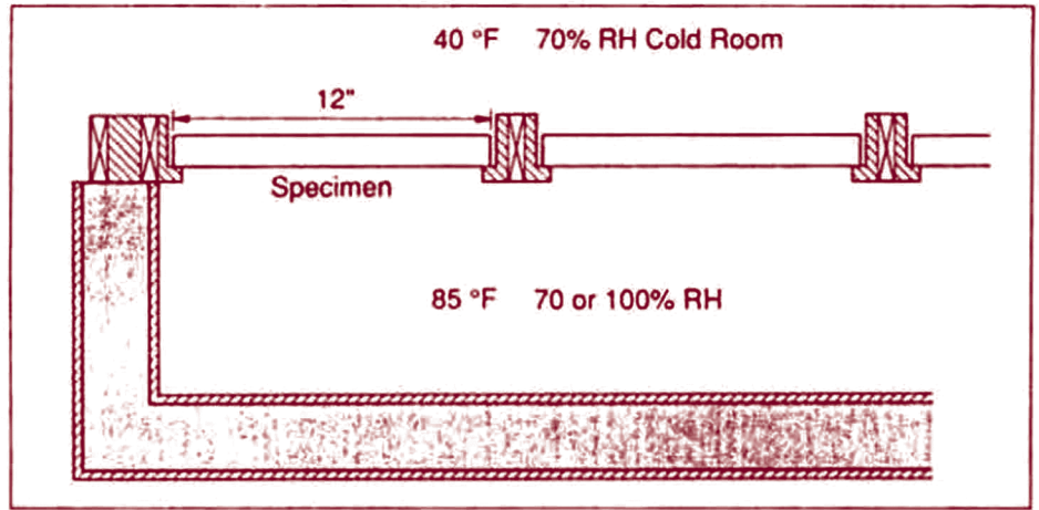
Figure 1 Sketch of specimens in wetting apparatus.
