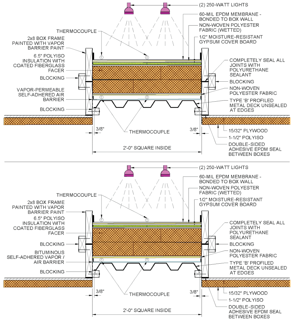
Figure 8 – Second test assemblies.
