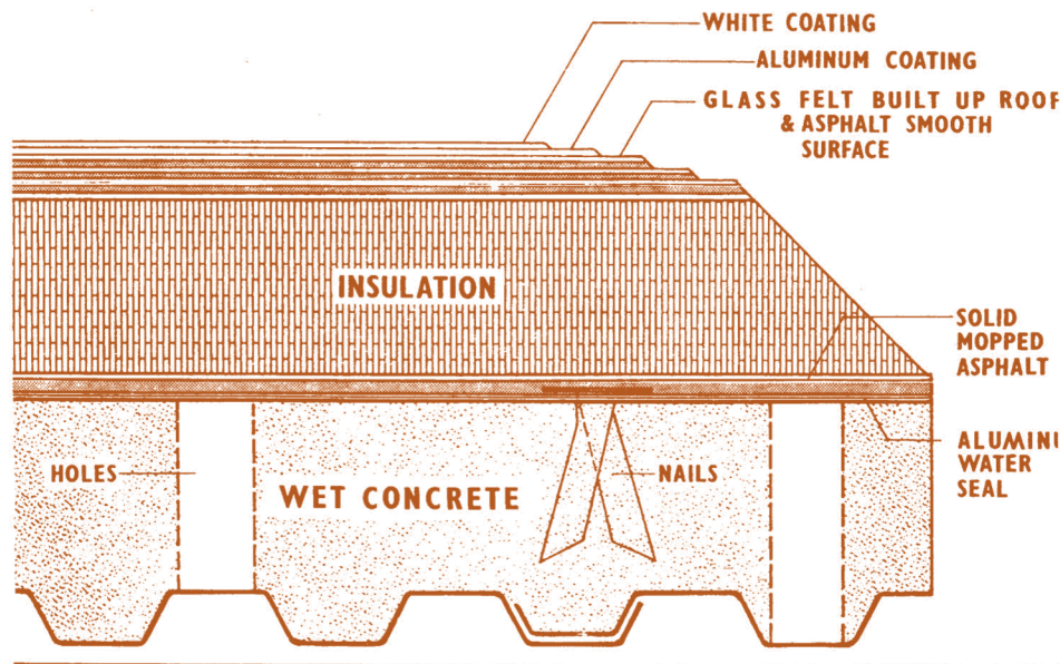
Figure 6 Glass felt built-up roof
