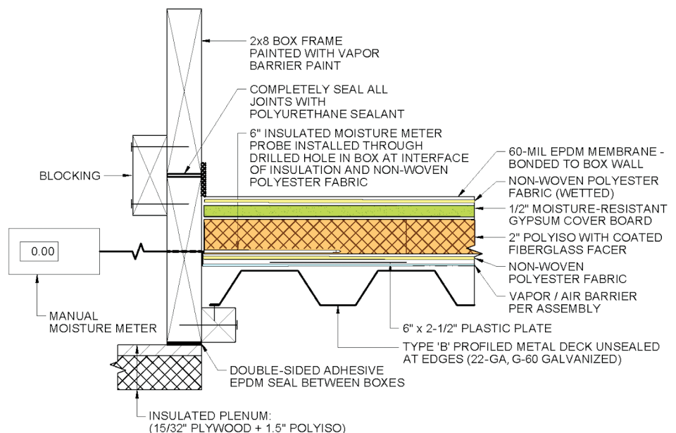
Figure 9 – New test panel assembly.
