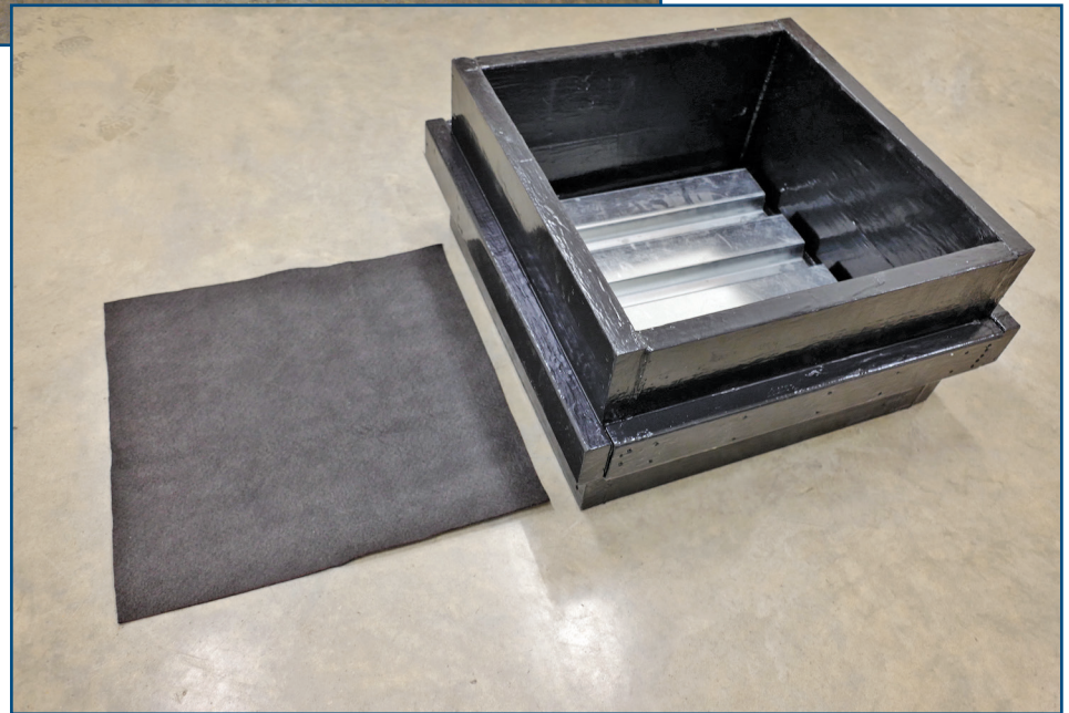
Figure 5 – Non-woven polyester fabric and test panel. The panel box is fully coated in a vapor-impermeable paint.
