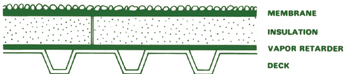
FIG. 1 —Cross section of a compact roofing system.
