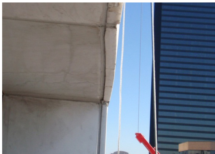
FIGURE 14. Representative view of bowed facade panel.
