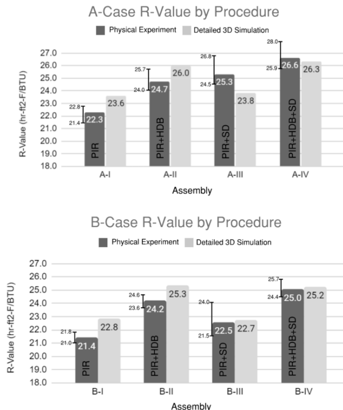
FIGURE 11. Comparative R-value results.
