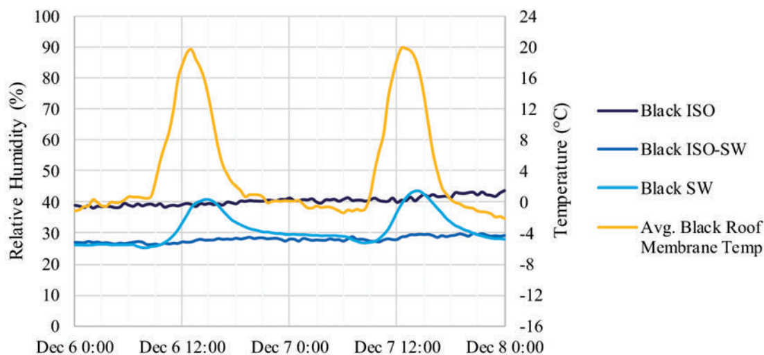
Figure 18 – Sample daily RH levels for different insulation arrangements in winter 2017.
