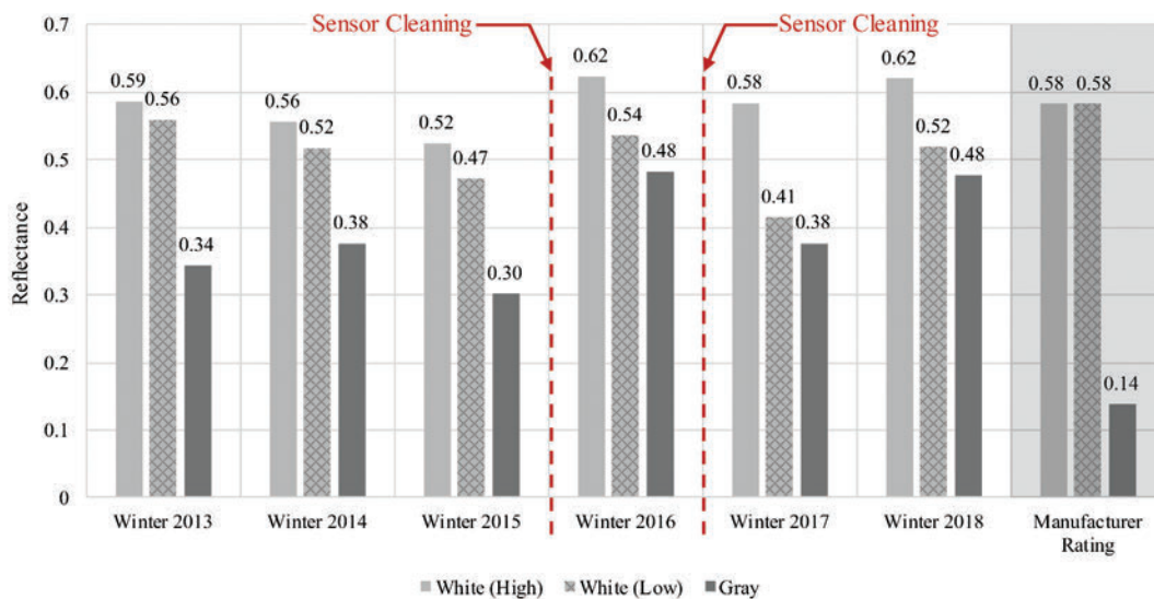
Figure 6 - Average reflectance of membrane between December 21 and March 20 over the six-year monitoring period. Note when the sensors were cleaned (March 2015 and December 2016), indicated with red dashed lines.
