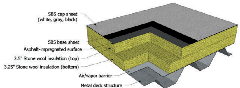
Figure 2 – Stone wool roof assembly; two layers of stone wool insulation. Total nominal R-value (hr·ft 2 ·°F/Btu) = R-21.9 (top layer = R-9.5, bottom layer = R-12.4)
