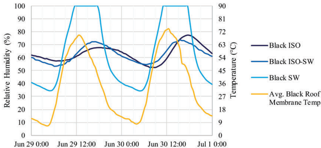
Figure 17 – Sample daily RH levels for different insulation arrangements in summer 2017.
