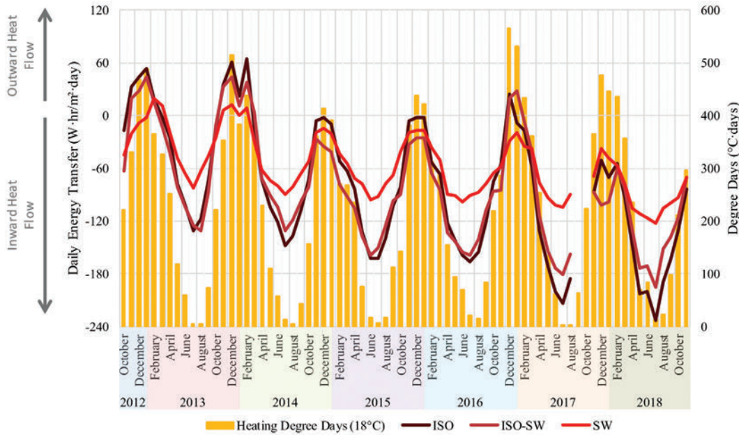
Figure 13 – Graph of monthly average degree daily energy transfer by insulation arrangement.
