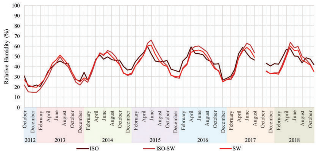
Figure 16 – Monthly average RH levels below the insulation for each insulation arrangement.
