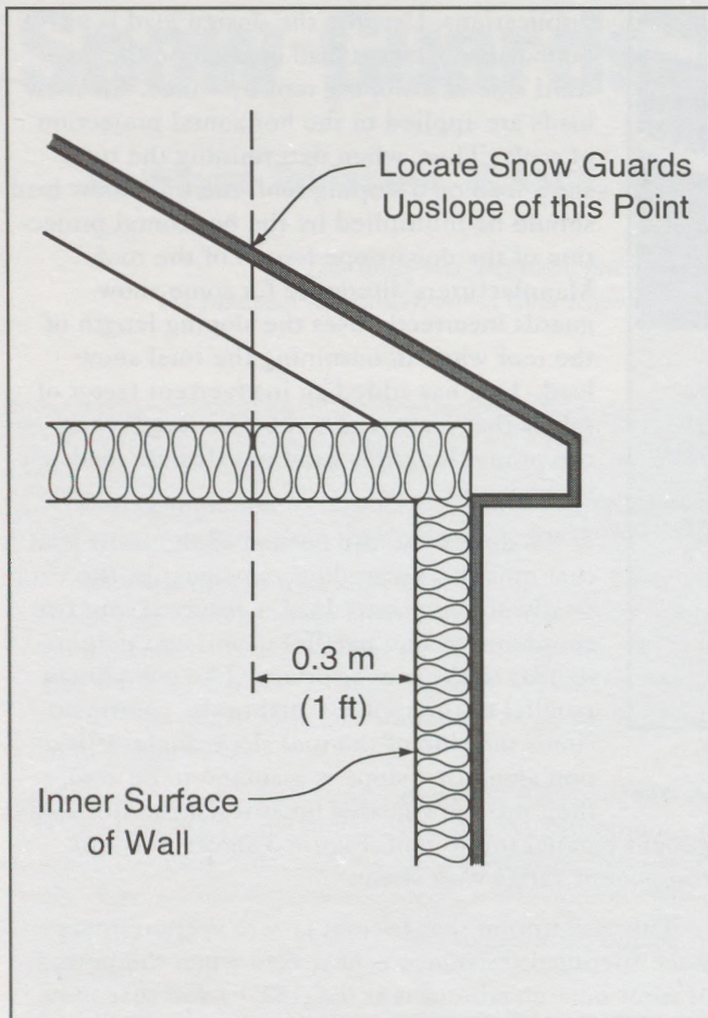
Figure 4: Snow guards should be kept some distance above eaves to keep ice from accumulating on them.
