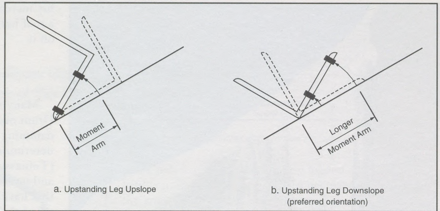
Figure 10: Alternative orientations of the long aluminum angle snow guards. By placing the upstanding leg downslope, a stronger system was achieved.
