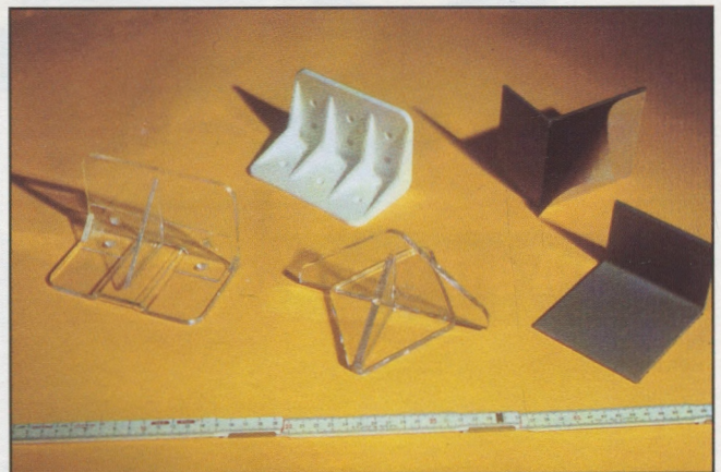
Figure 1: Examples of adhesively-attached snow guards.
