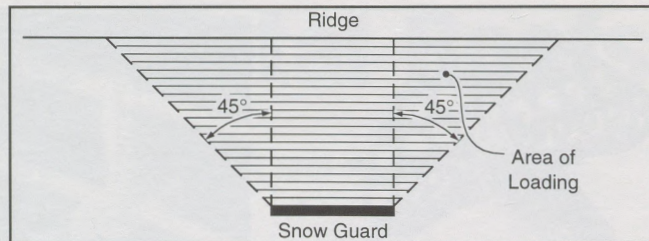
Figure 6: Loaded area for an isolated snow guard.
