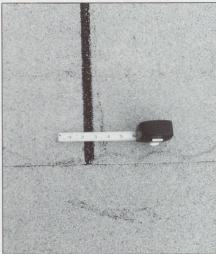
Polyester reinforced modified bitumen cap sheet exhibiting shrinkage at end lap.
