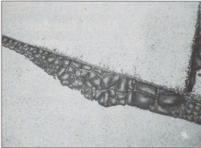
Alligatoring of exposed asphalt bleed-out along edge of cap sheet.
