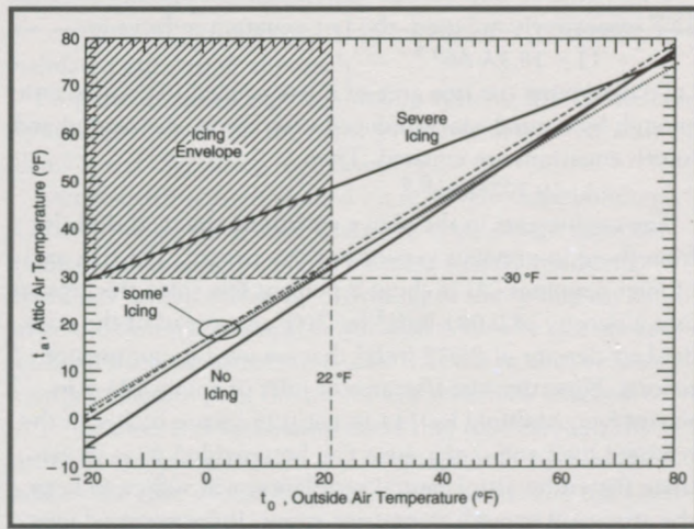
Figure 8: Lines of best fit for the three roofs shown in Figures 5-7, along with similar lines (dashed) for two other roofs also having "some" icing problems.
