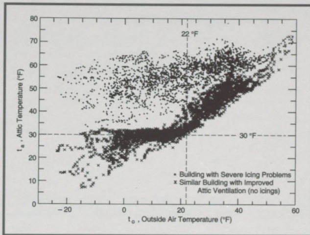
Figure 10: Attic temperature vs. outside air temperature for a building with severe icing problems and a similar building with improved attic ventilation experiencing no icing problems.
