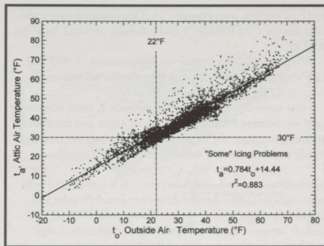
Figure 6: Attic temperature vs. outside air temperature for a roof experiencing "some" icing problems.
